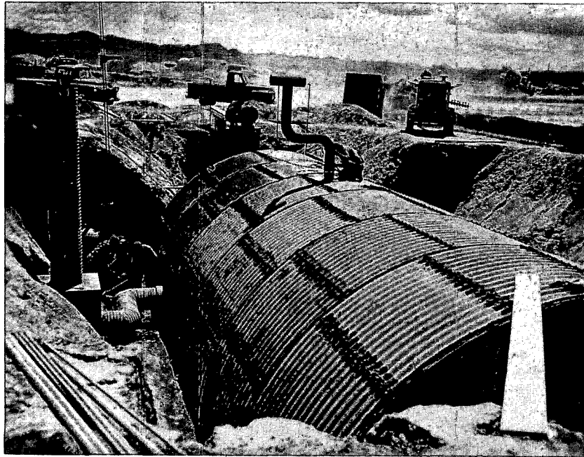
Fig. 7—Overall view before backfilling, structure 3.3c.
